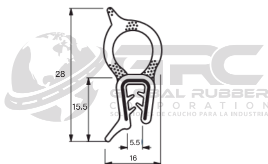
Perfil Burlete Alambrado EM04
